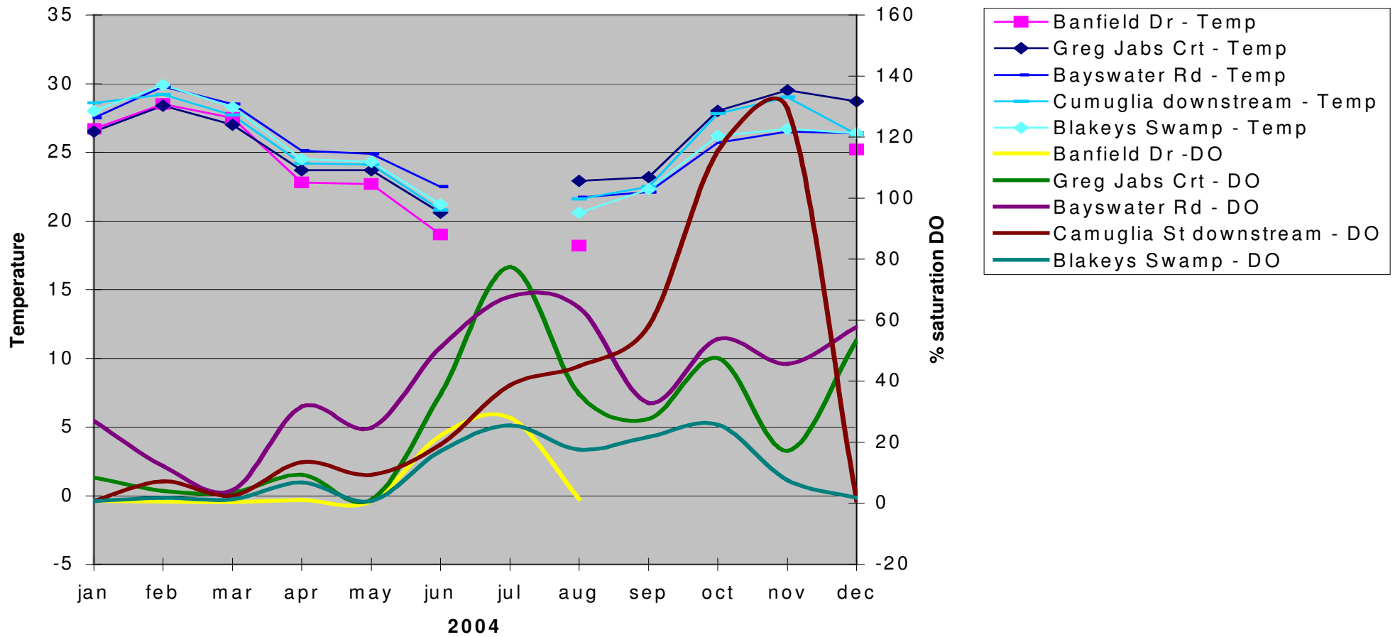
2004 - dissolved oxygen (DO) compared to water temp
